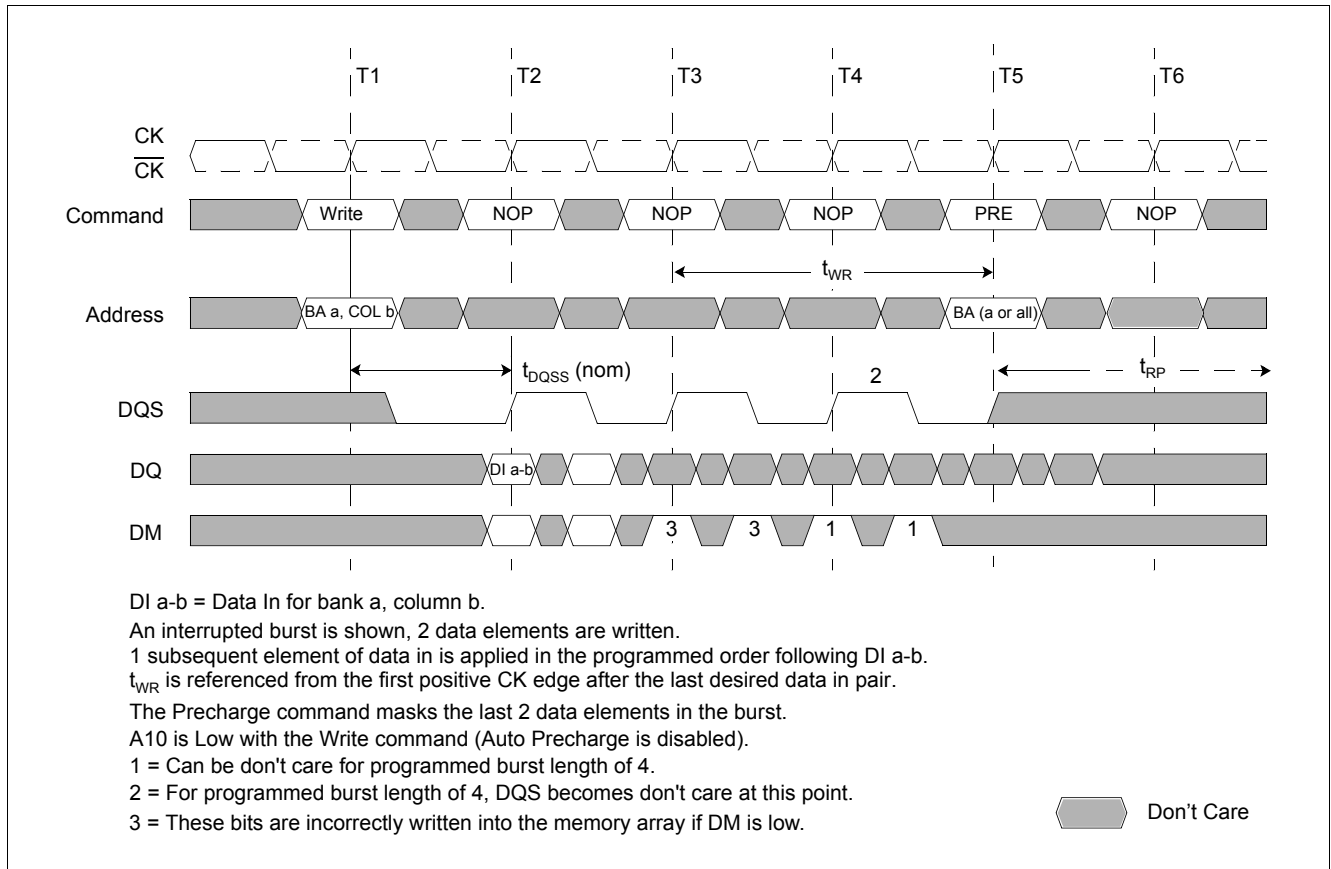
Figure 29 Write to Precharge: Nominal DQSS (2-bit Write), Interrupting (Burst Length = 4 or 8)
