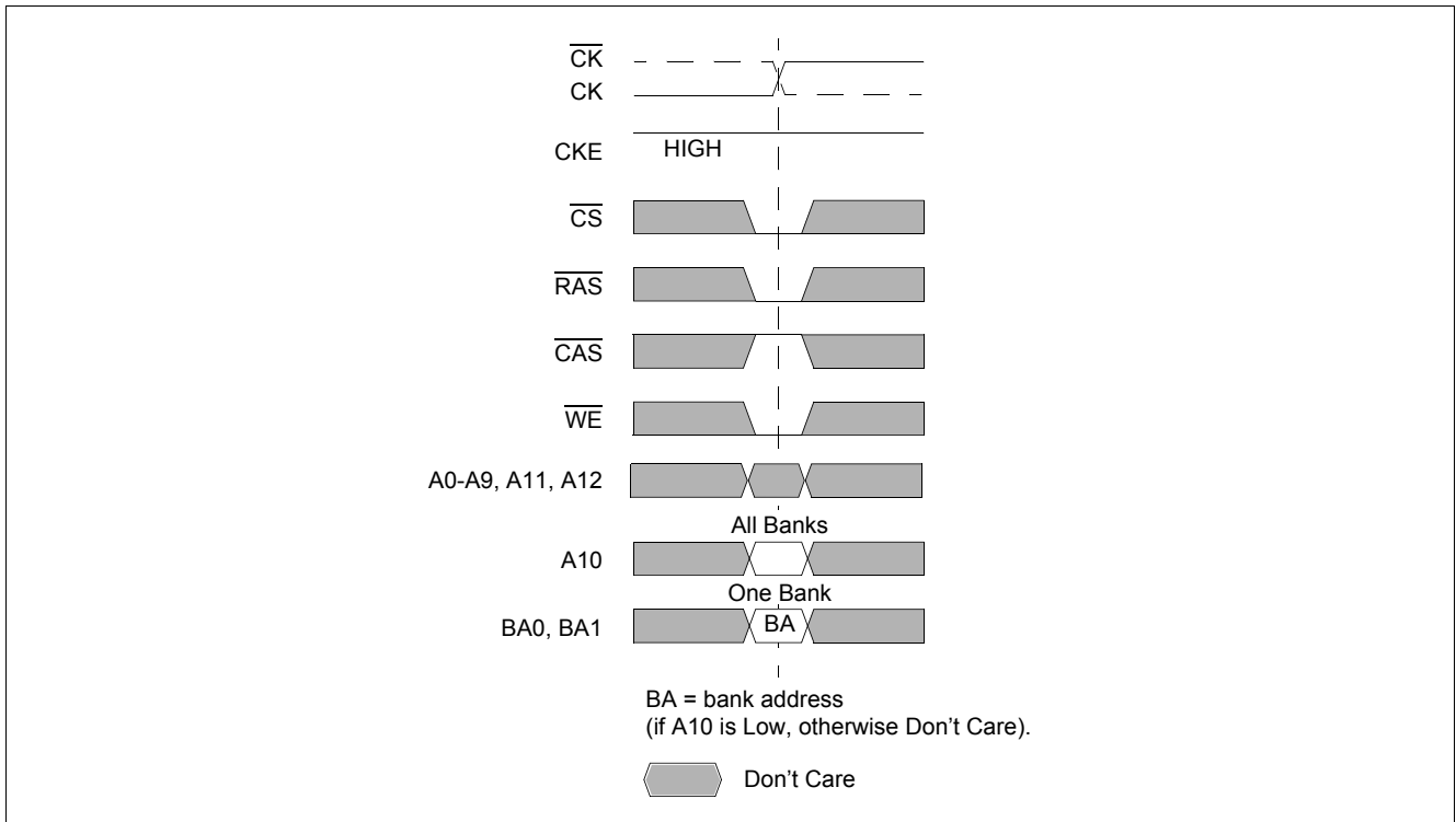
Figure 30 Precharge Command
