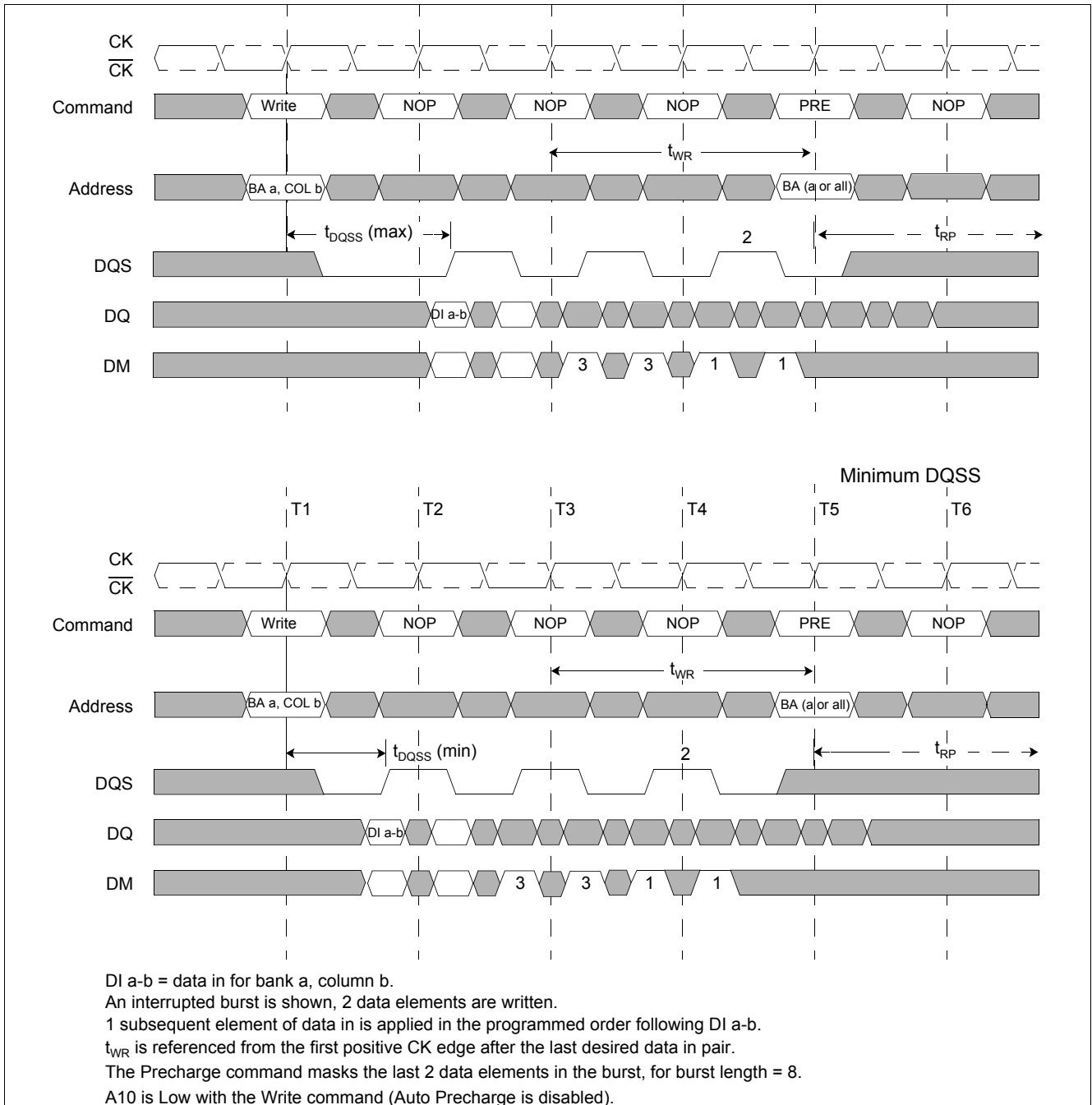
Figure 27 Write to Precharge: Interrupting (Burst Length = 4 or 8)
