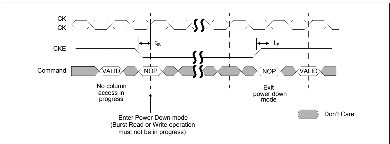
Figure 31 Power Down
