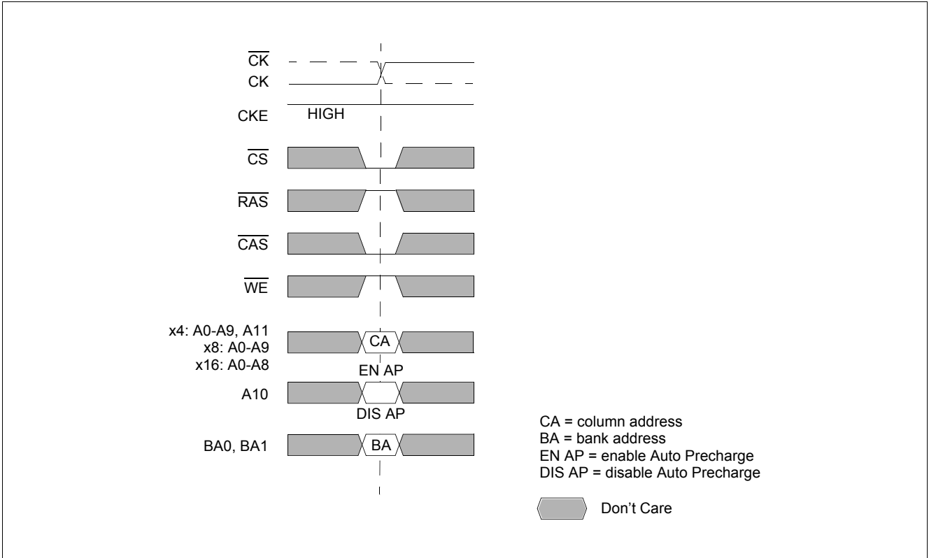
Figure 9 Read Command
